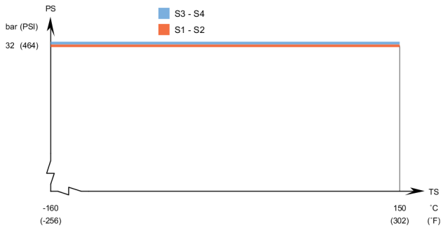
CD100 - CRN approval pressure/temperature graph
