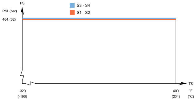
CD100 - UL approval pressure/temperature graph
